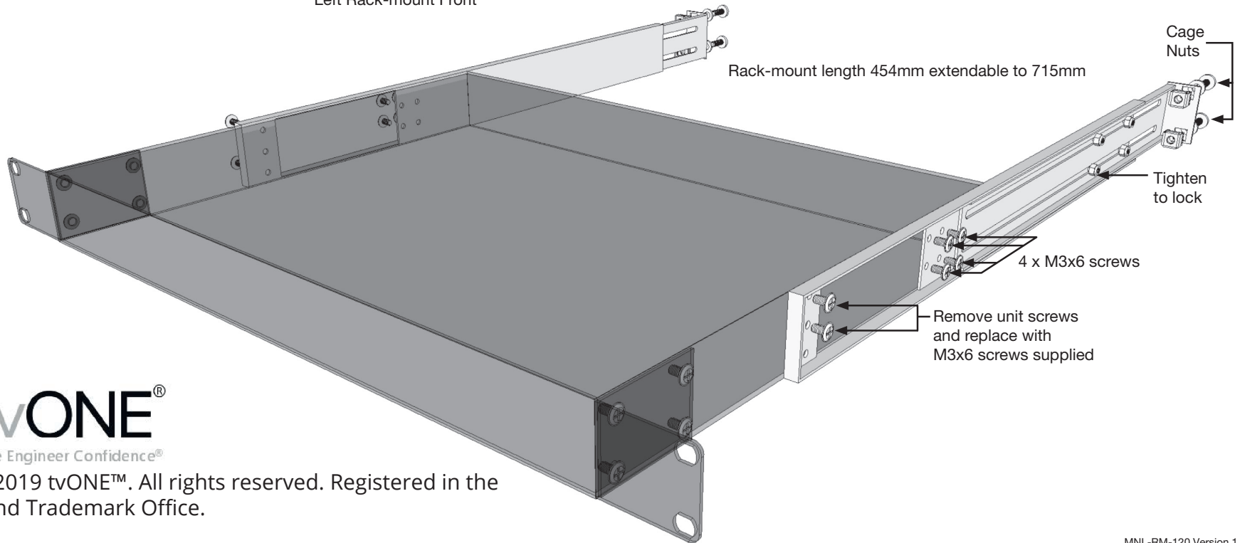
Left Rack-mount Front
